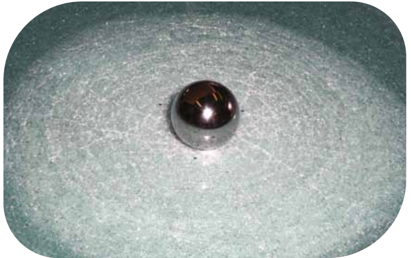
Impact testing, EN356.
